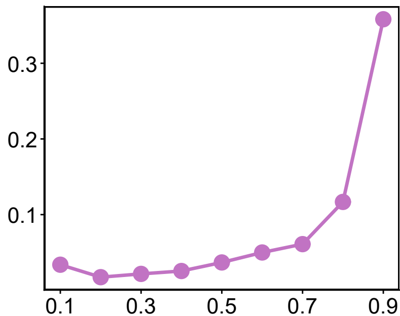
Collective variance
