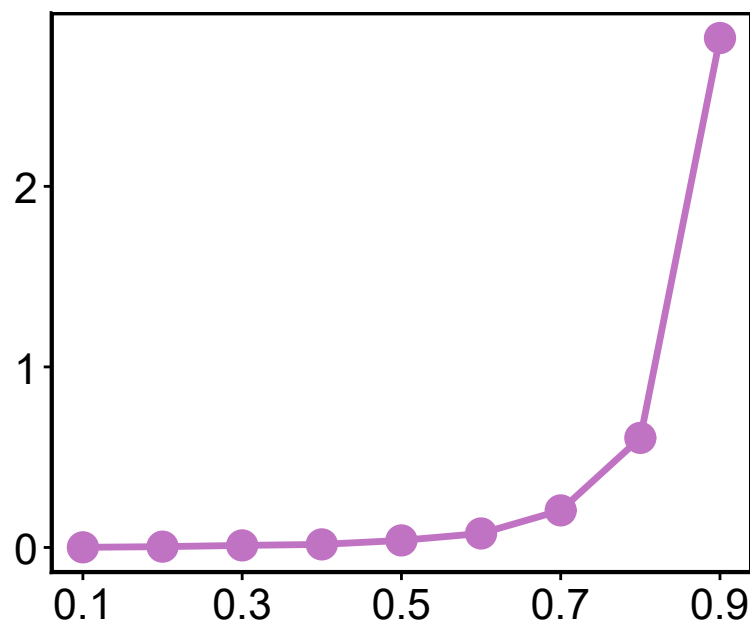
Collective bias
