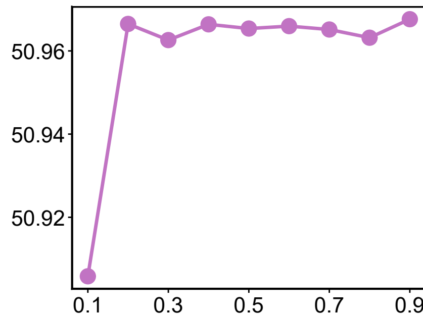
Interest Diversity
