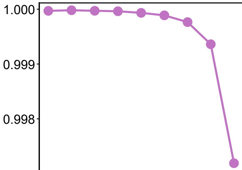
Collective accuracy
